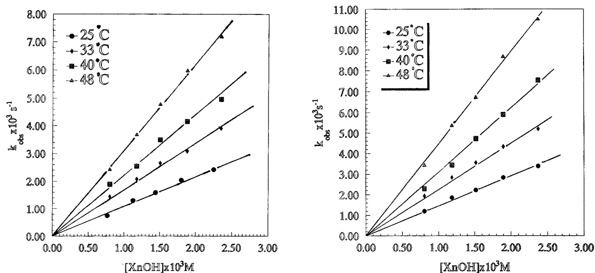
Figure 1. Linear correlations of k_{\text{obs}} vs [\text{XnOH}] in the reductions of \text{Xn}^+ by BNAH (0.04 mM) (left) and HEH (0.04 mM) (right) at 25, 33, 40 and 48 °C
